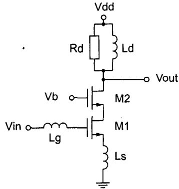
Fig. 2. Schematic diagram of the preamplifier.
