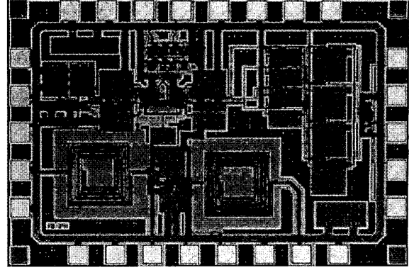
Fig. 7. Chip micrograph.
